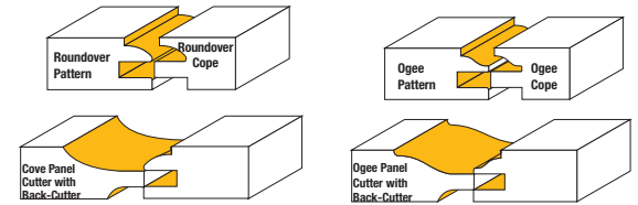
Roundover Rail & Stile Set ITEM # 02011 Ogee Rail & Stile Set ITEM # 02012
