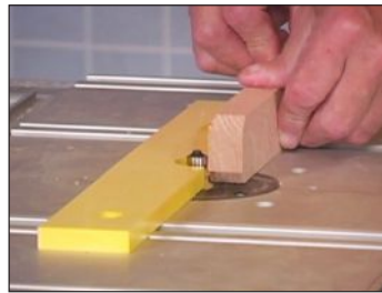
STEP 3: Route the bead on the face frames for decorative purposes
