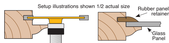
The slot cutter cuts a slot for the rubber panel retainer
